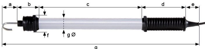
Abmessungen in mm | Dimensions in mm
